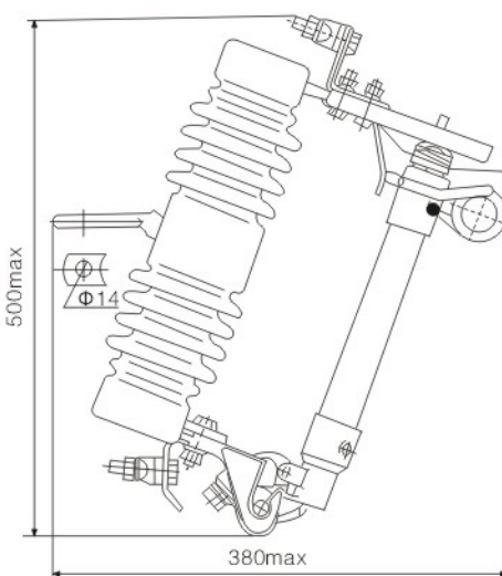
PRW8-(15-27)/100型熔断器 PRW8-(15-27)/100 dropout fuse
