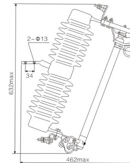
PRW8-40.5/100型熔断器 PRW8-40.5/100 dropout fuse
