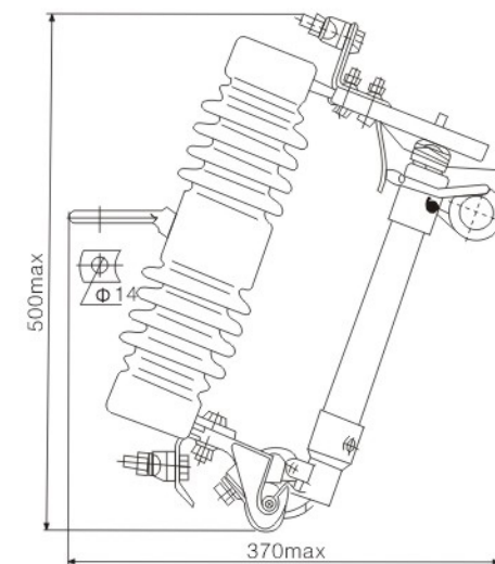
PRW8-(15-27)/200型熔断器 PRW8-(15-27)/200 dropout fuse
