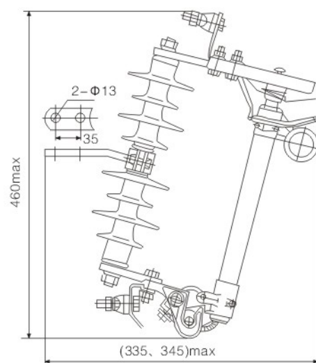
PRHW10-12/(100, 200)型熔断器 PRHW10-12/(100,200)dropout fuse
